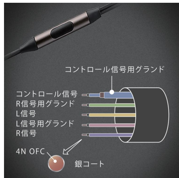
Noiseless Hybrid Wiring
